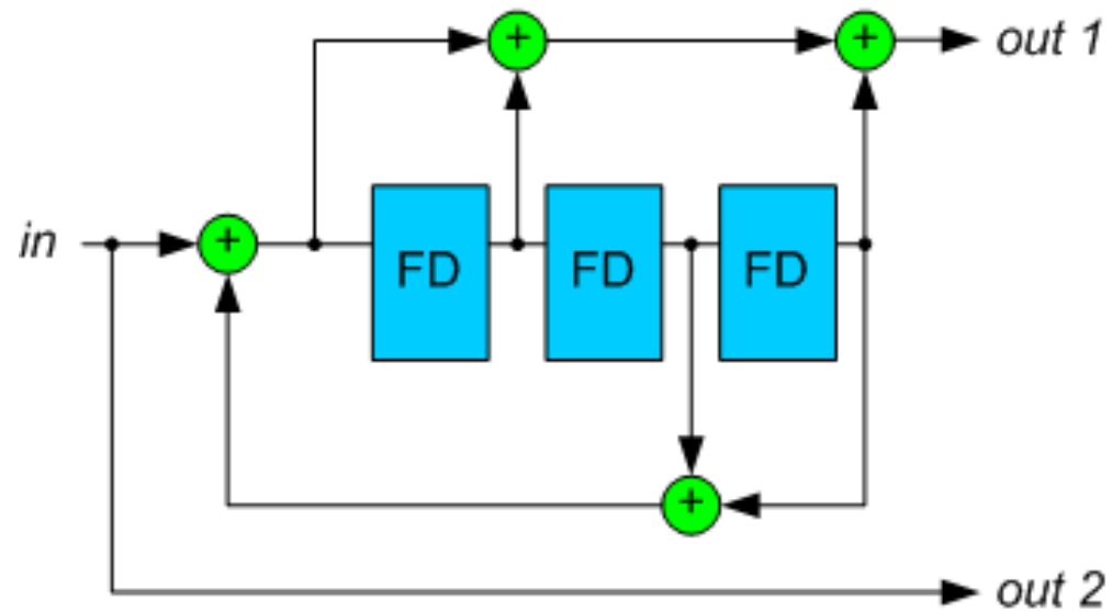
Figure 2. A recursive convolutional encoder.
