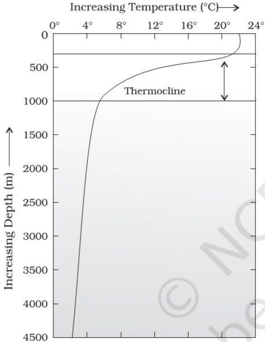
Figure 13.3 : Thermocline
